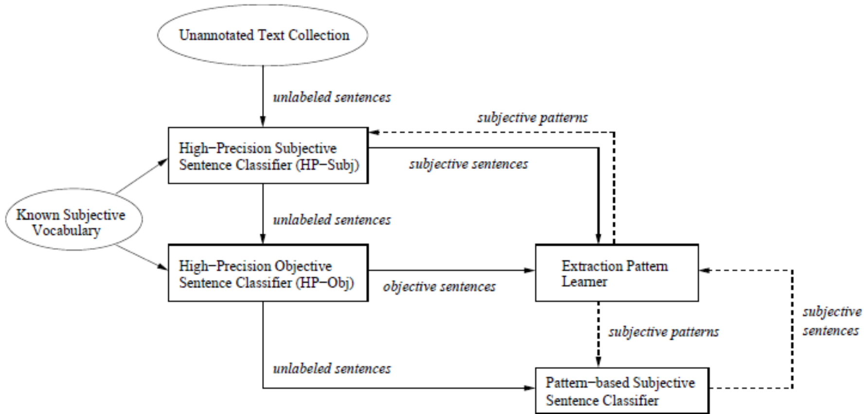
Figure 1: Bootstrapping Process
